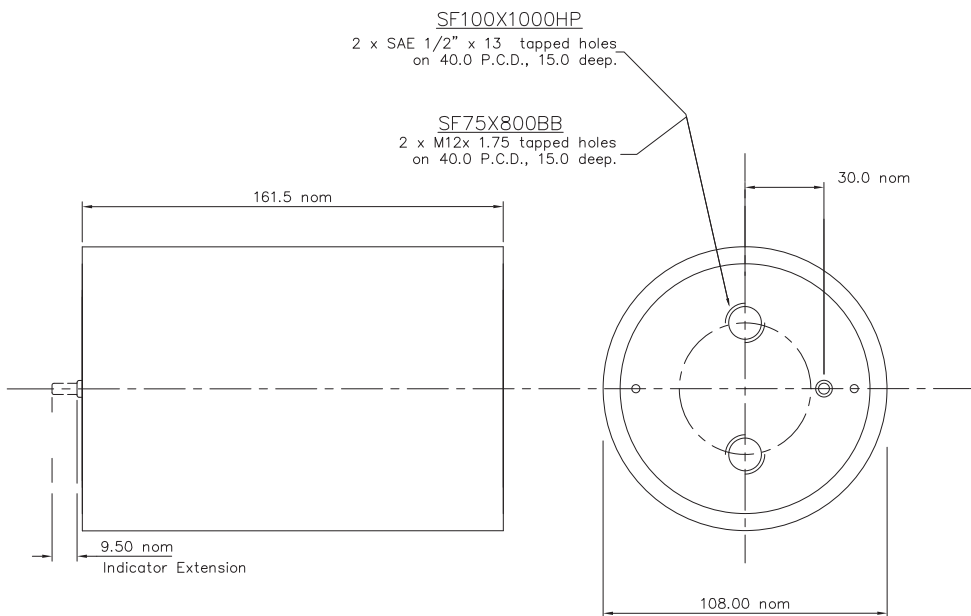
Dimensions (mm) - SF75X800BB and SF100X1000HP, Blade contact
