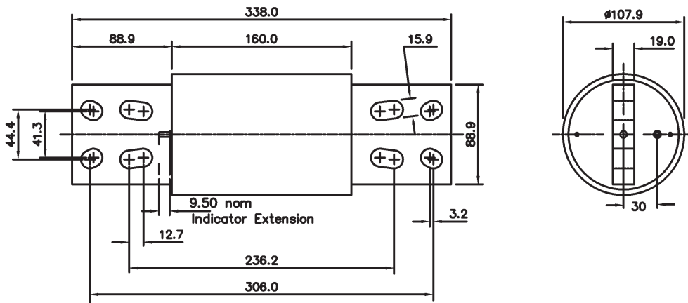
Dimensions (mm) - SF100X1000 , Blade contact
