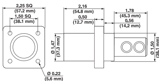
MALE DOUBLE SET SCREW PANEL RECEPTACLE
