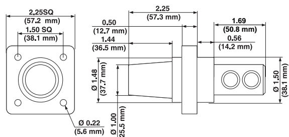
FEMALE DOUBLE SET SCREW PANEL RECEPTACLE
