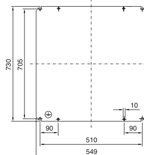
Mounting plate
