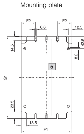
5 For 125 mm wide mounting plates, attachment is in the centre only
