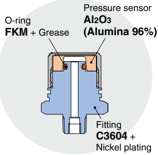
Port size R1/4 (with M5 female thread)
