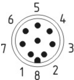
Contact arrangement
