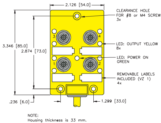
4-Port with Integral Home Run Cable
