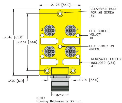
4-Port with multifast Home Run Connector
