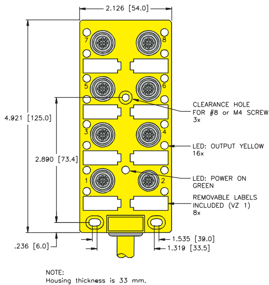
8-Port Integral Home Run Cable
